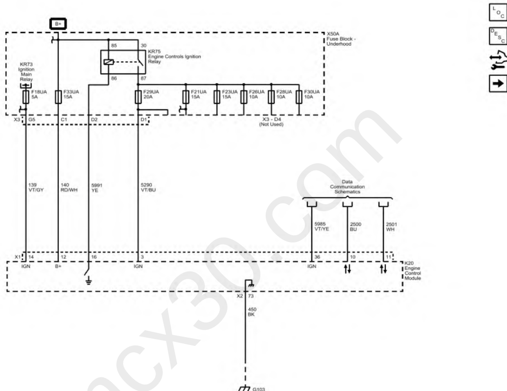
Fig. 1: Module Power, Ground, Serial Data, and MIL (Chevrolet with 2H0). Courtesy of GENERAL MOTORS COMPANY
