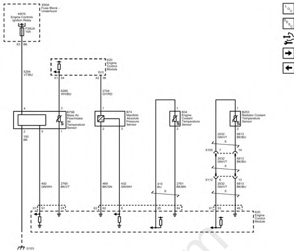
Fig. 4: Engine Data Sensors - Pressure and Temperature (Chevrolet with 2H0). Courtesy of GENERAL MOTORS COMPANY
