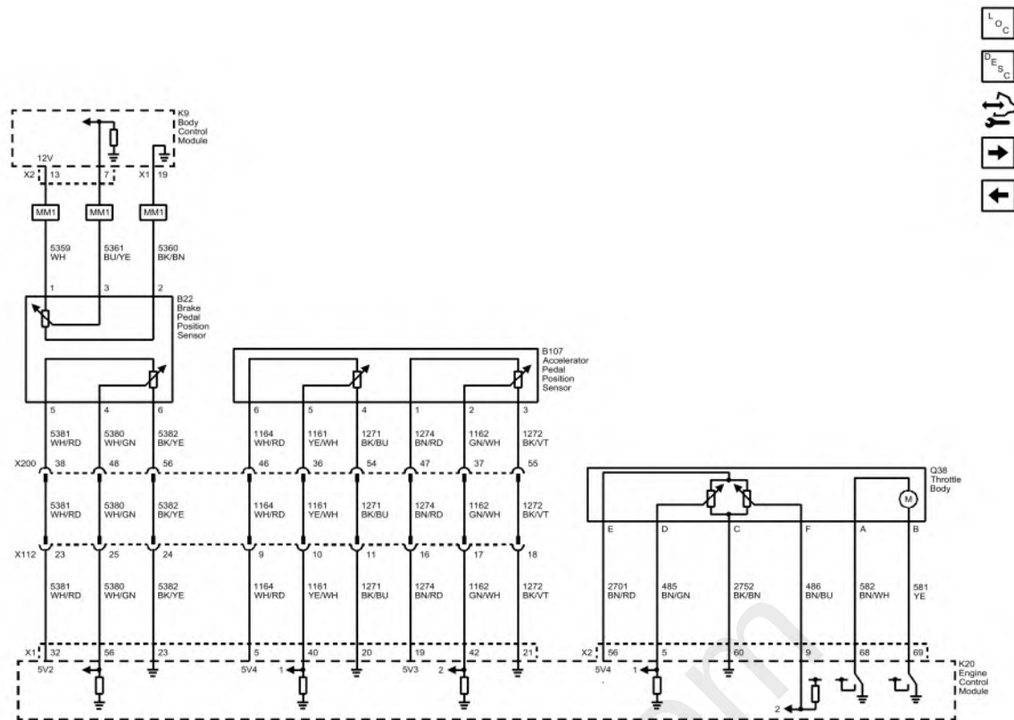
Fig. 6: Engine Data Sensors - Throttle and Brake Sensor Controls (Chevrolet with 2H0). Courtesy of GENERAL MOTORS COMPANY
