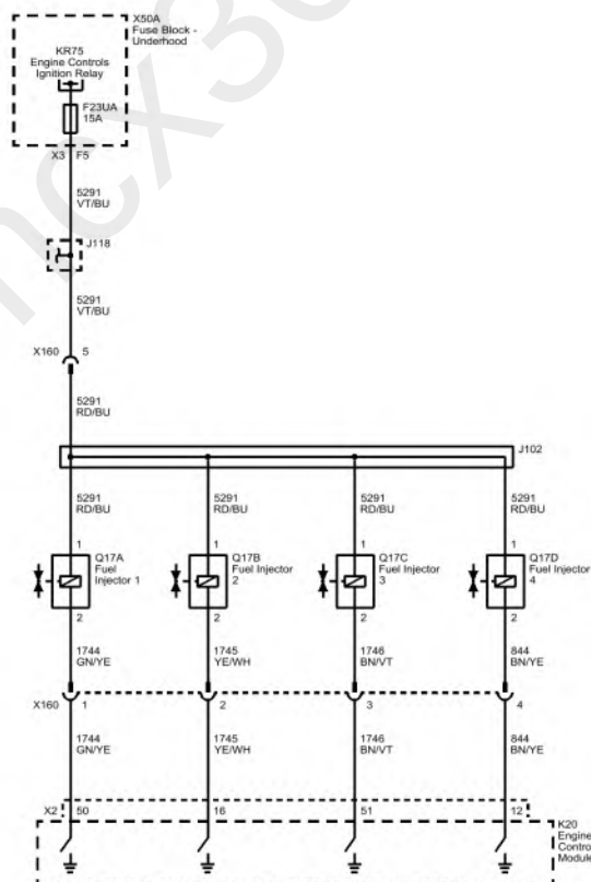
Fig. 11: Fuel Controls - Fuel Injectors (Chevrolet with 2H0). Courtesy of GENERAL MOTORS COMPANY
