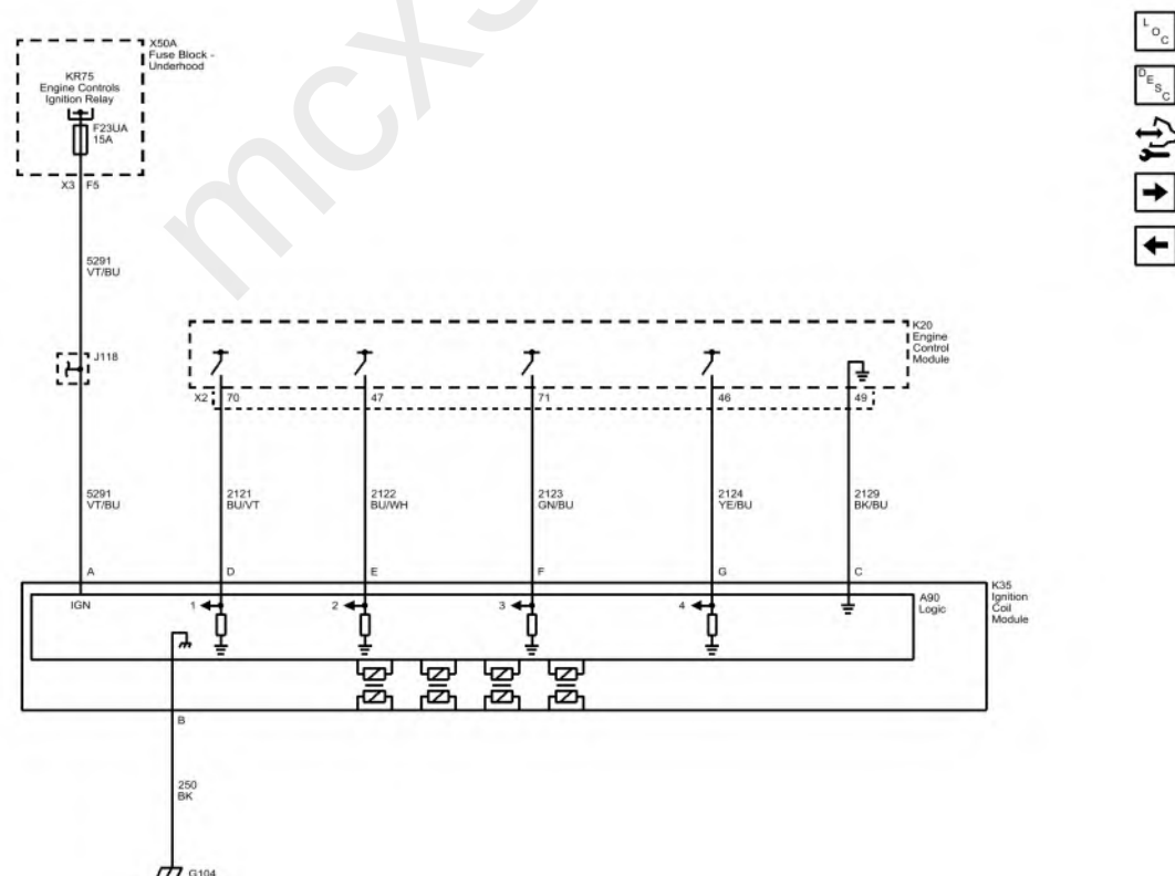
Fig. 7: Ignition Controls - Ignition Coil (Chevrolet with 2H0). Courtesy of GENERAL MOTORS COMPANY
