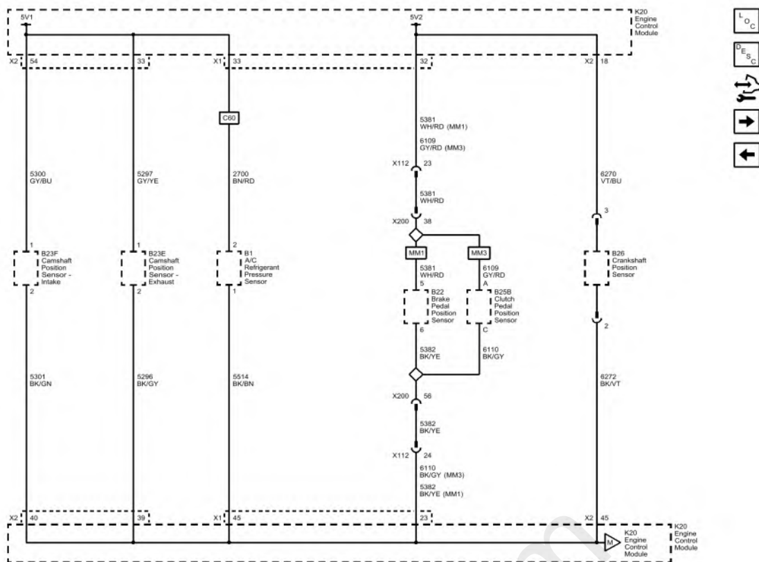
Fig. 2: 5V1, 5V2, and Low Reference Bus (Chevrolet with 2H0, page 1 of 2) Courtesy of GENERAL MOTORS COMPANY
